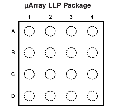
Top View (Bump_side down) Order Number LM4906GR See NS Package Number GRA16A
